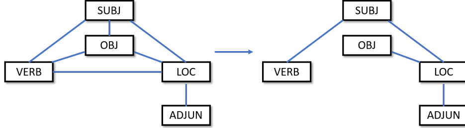
Figure 4.2: An example of reducing full CRF into tree CRF.
