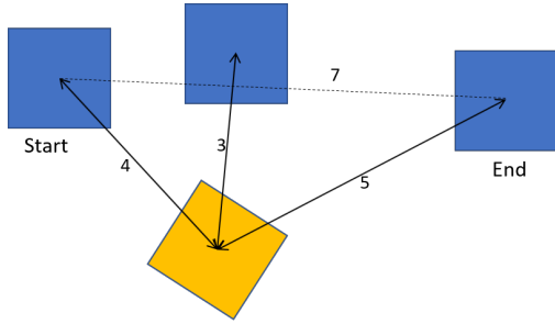
Figure 5.15: A demonstration of evaluation algorithm for Slide Past. We could check the distance between two objects at the beginning, at the end, and one intervening frame.
