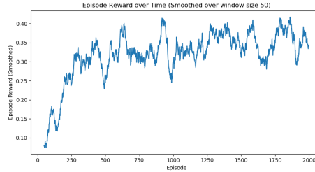
Figure 5.24: Average rewards of ACTOR-CRITIC on discrete space for Slide Around after 2000 episodes. Each state does not have quantized progress
