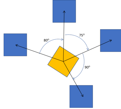
Figure 5.16: A demonstration of evaluation algorithm for Slide Around. We could check the total non-overlapping angle of the movement the moving object makes around the static object. It is 245^\circ here.
