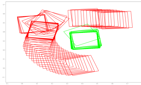
Figure 2.6: An recorded demonstration of "Move A around B" projected onto the 2-D simulator. A is projected as a red square, B as a green square. In this image, the simulator is in offline mode, and only used to show the trajectory of a recorded demonstration.
