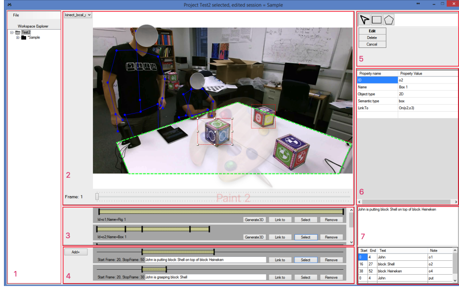
Figure 3.2: ECAT GUI. The left panel allows annotators to manage their captured and annotated sessions. Recognized human rigs are displayed as blue skeletons. Objects of interest are marked in color in the scene view. Here shows an example of collecting data for human activity corpus
