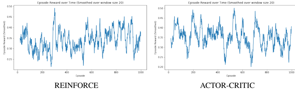
Figure 5.21: Same configuration as in Figure 5.20 but with 3 – action hybrid setup.
