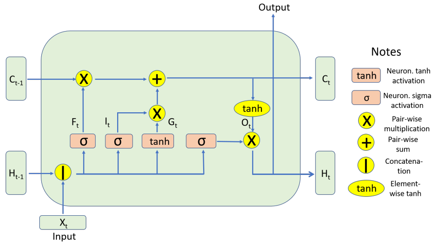
Figure 2.4: Architecture of an LSTM node. Note the color code for simple (pairwise, or element-wise) operations is yellow, for neural operation is light orange.
