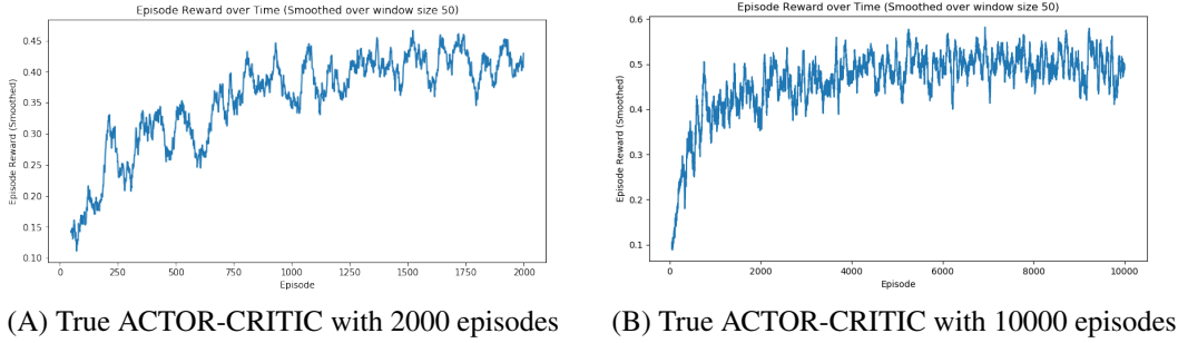
Figure 5.22: Average rewards of ACTOR-CRITIC on discrete space for Slide Around after 2000 and 10000 running episodes.
