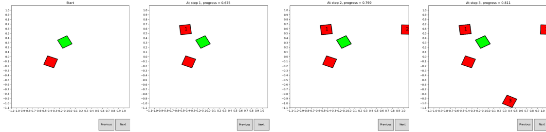
Figure 2.7: A demonstration in interactive mode using continuous learned progress function. At each step, the simulator looks for the best action that can increase the progress value. The progress values at the top improve from 0 to 0.675 to 0.769 to 0.811
