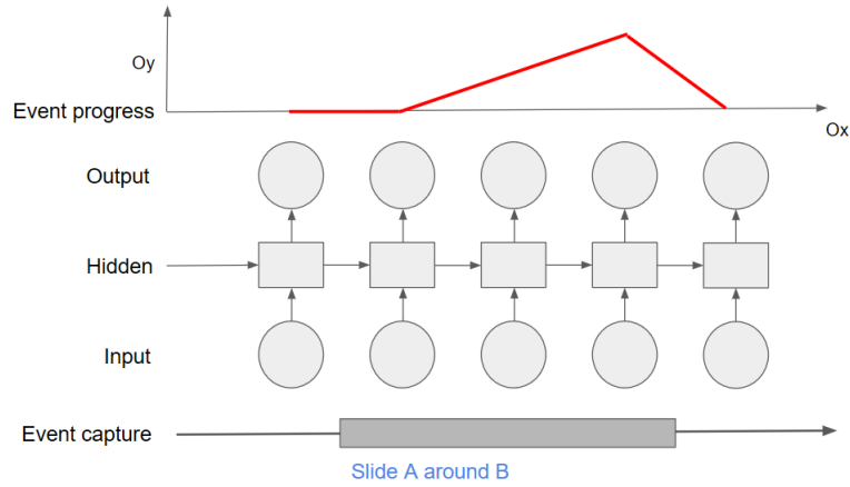
Figure 2.5: LSTM network producing event progress function
