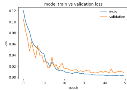
Figure 5.9: MSE with half the data and qualitative features.
