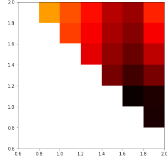
Figure 5.18: The PCC values for different combinations of \alpha_1 and \alpha_2 for Slide Around. The best value combination is when \alpha_1 = 1.1 and \alpha_2 = 1.7
