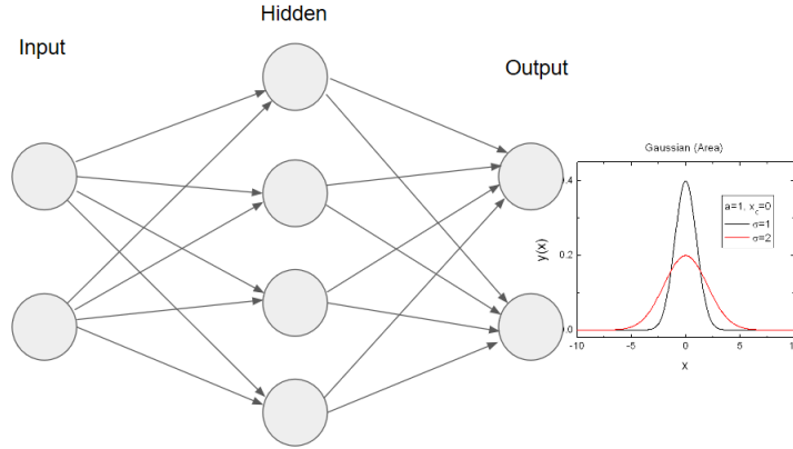
Figure 5.3: An ANN architecture producing Gaussian policy
