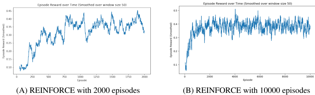
Figure 5.23: Average rewards of REINFORCE on discrete space for Slide Around after 2000 and 10000 running episodes.
