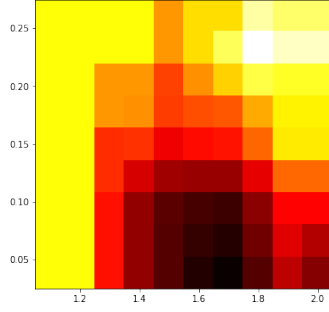
Figure 5.17: The PCC values for different combinations of angle_diff and threshold for Slide Next To. The best value combination is when angle_diff = 0.05 and threshold = 1.7.
