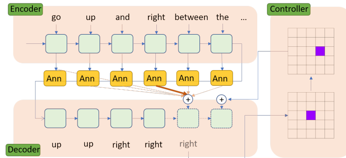
Figure 6.3: Seq2Seq model with controlling loop from the visual state to the input of the decoder)
