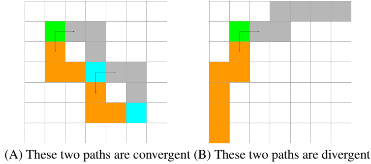
Figure 6.4: While the internal evaluation is agnostic to convergent versus divergent paths, external evaluation measure accounts for this distinction. Starting position is color green , intercepting positions are blue , candidate path follows the gray cells, and reference path follows orange cells
