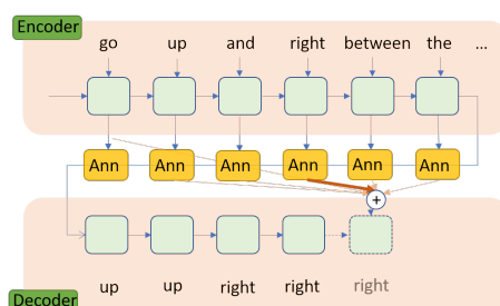
Figure 6.2: Attention RNN model (Bahdanau additive attention style)
