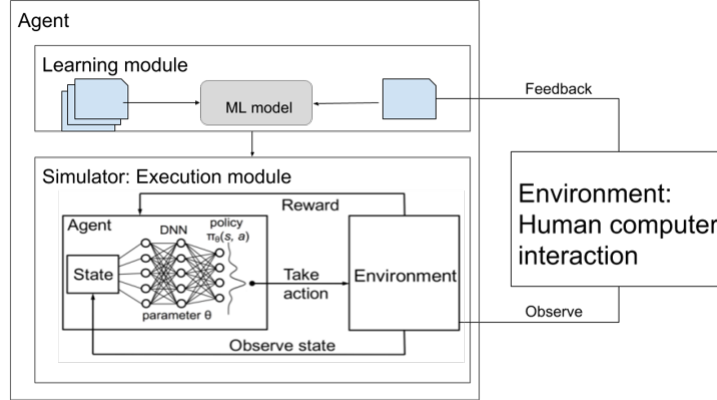
Figure 1.2: Reinforcement learning framework
