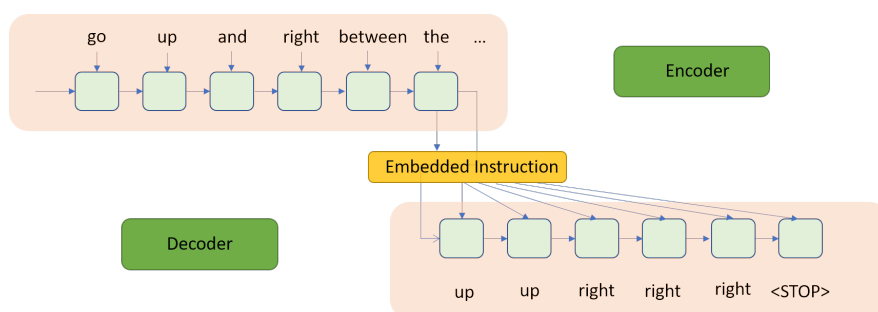
Figure 6.1: Encoder-decoder model
