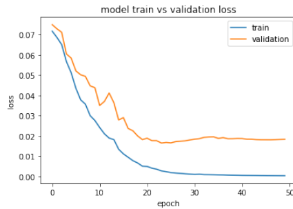
Figure 5.8: MSE with half the data and quantitative features.
