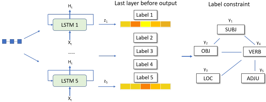
Figure 4.1: An array of LSTM models produce an array of output values, each corresponds to a sentence slot classifier. The values at the last layer of each LSTM is a probability distribution (in practices, their logarit values). These values are fed into CRF as values of x in Equation 4.3
