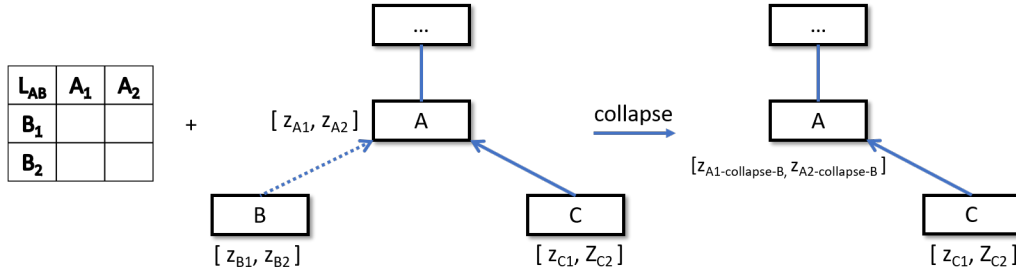
Figure 4.3: Collapsing an edge between nodes A and B into one node when calculating Z for updating. Note that B needs to be a leaf node
