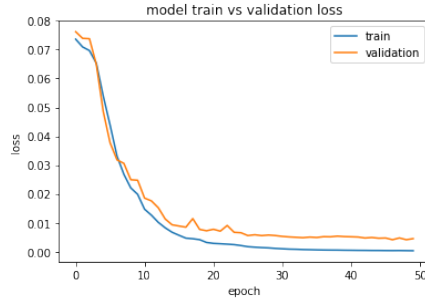
Figure 5.6: MSE with all data and quantitative features.
