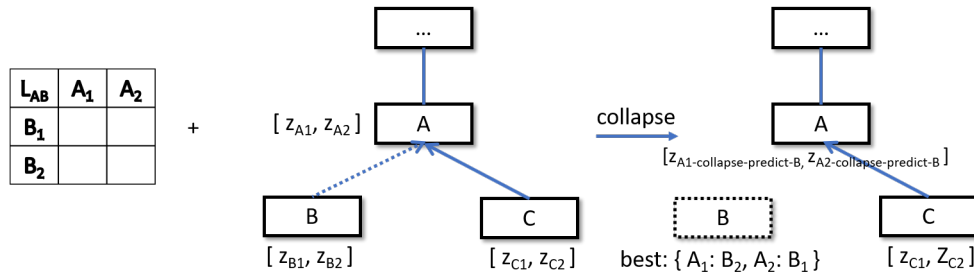
Figure 4.4: Collapsing an edge between nodes A and B into one node when predicting the output for a novel input.
