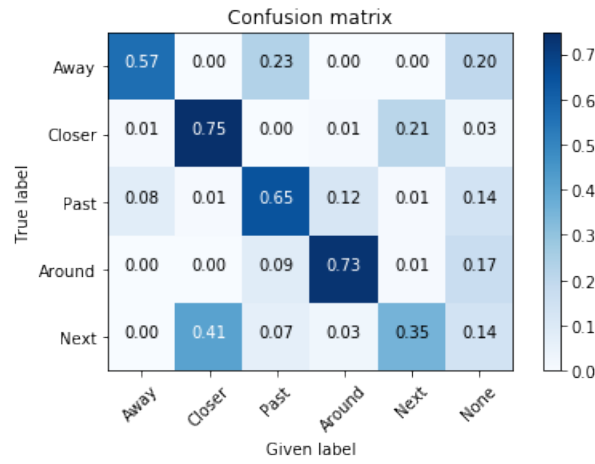
Figure 5.26: Confusion matrix of true labels versus human judged labels
