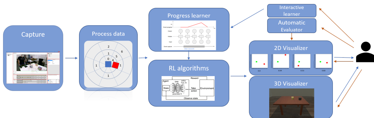
Figure 5.1: Learning workflow; blue arrows are data flows, brown arrows are evaluation flows
