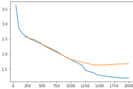
Figure 6.7: Perplexity of training (blue line) and evaluating (orange line) over 2000 steps (each step is one mini-batch update)
