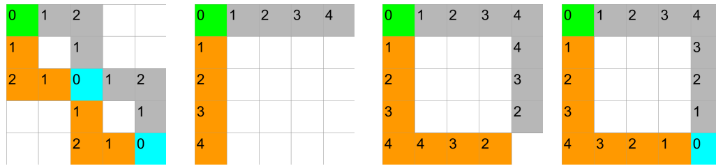
Figure 6.5: NEIGHBOR scores of some sample trajectories. The value of each cell is the distance to the closest cell on the other trajectory. Shared cells have the value of 0.
