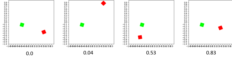
Figure 5.13: A bad demonstration of “Move the red block around the green block.” The value beneath each frame is value predicted by the progress learner.
